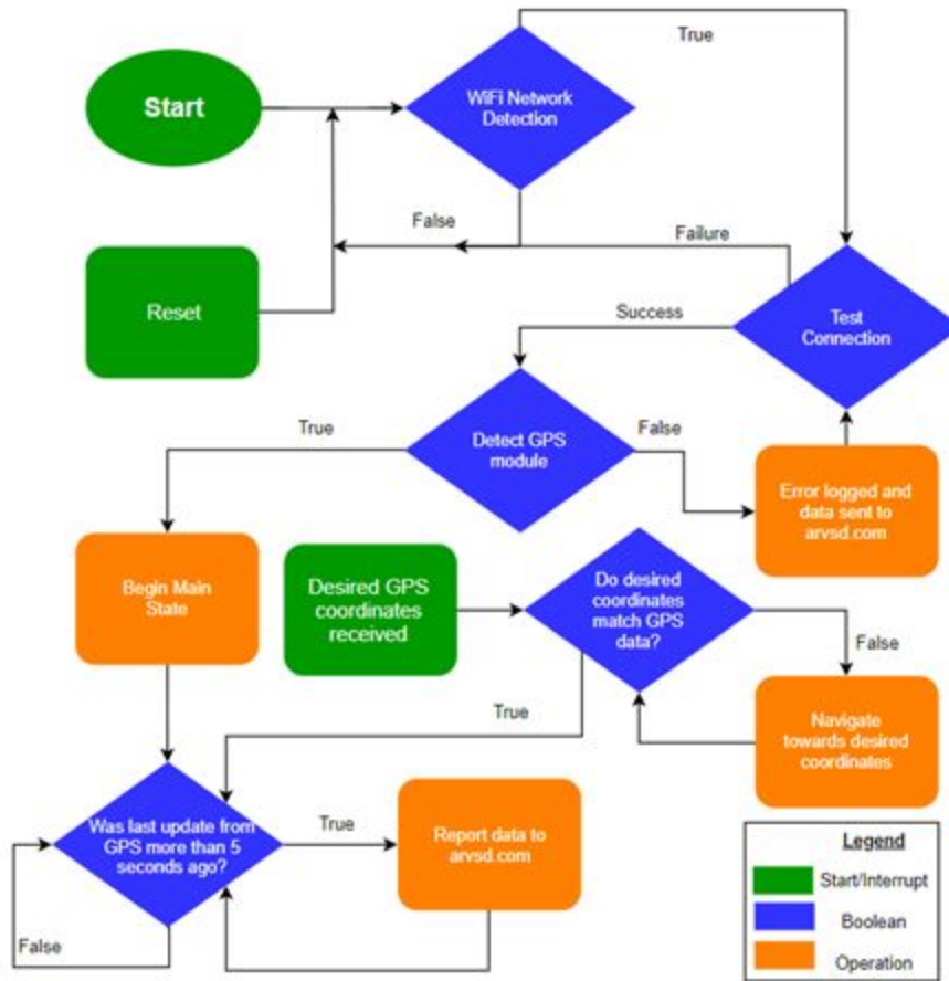
Figure 43: GPS Module Software Flowchart
