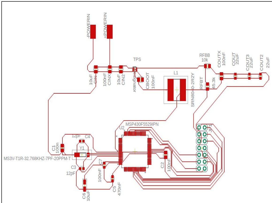
Figure 46: PCB Layout and Wired Connections
