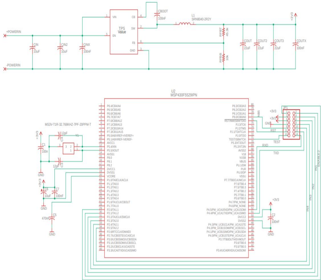
Figure 41: Overall Schematic using Eagle
